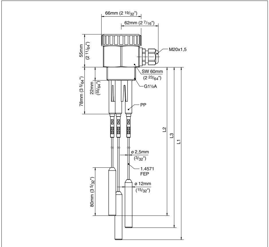
Fig. 7: Conductive multiple cable electrode EL 6
