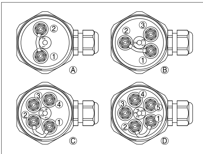
Fig. 4: Connection compartment of the probe - 220 kΩ resistance between terminals 1 and 2
