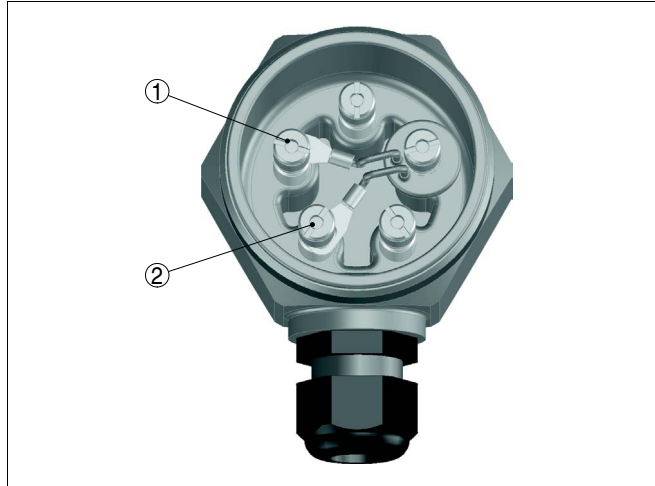
Fig. 6: Mounting of the component for line break monitoring
