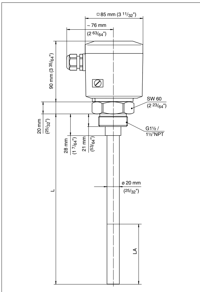
Fig. 23: VEGACAP 27, Modelo com rosca G1½ A
