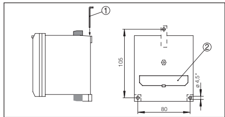
Abb. 10: Screw mounting
