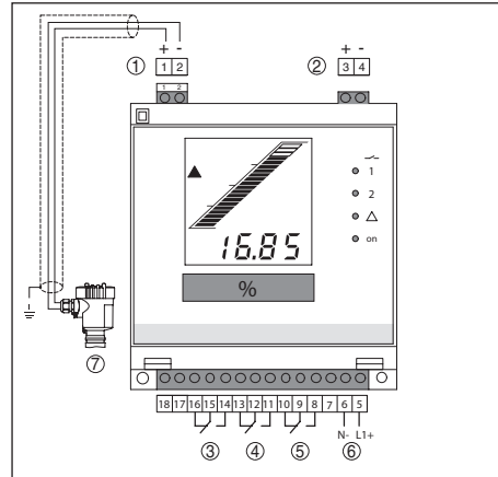
Abb. 12: Wiring plan with two-wire sensor
