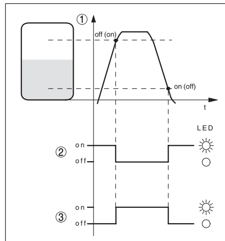
Abb. 14: Relay modes
