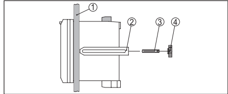
Abb. 9: Front panel mounting
