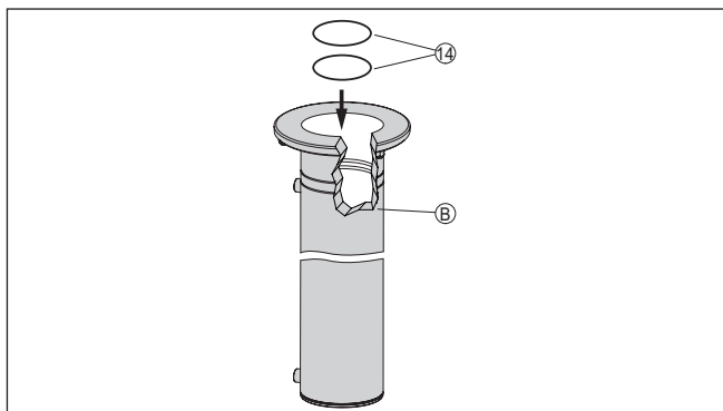
Fig. 2: Insert the sealing rings inside into the scintillator cooling
