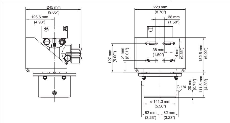
Fig. 20: Active water cooling system with housing cooling and housing cooling lid
