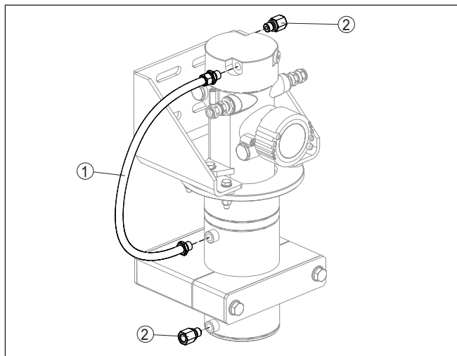
Fig. 17: Scintillator cooling - hoses and adapters
