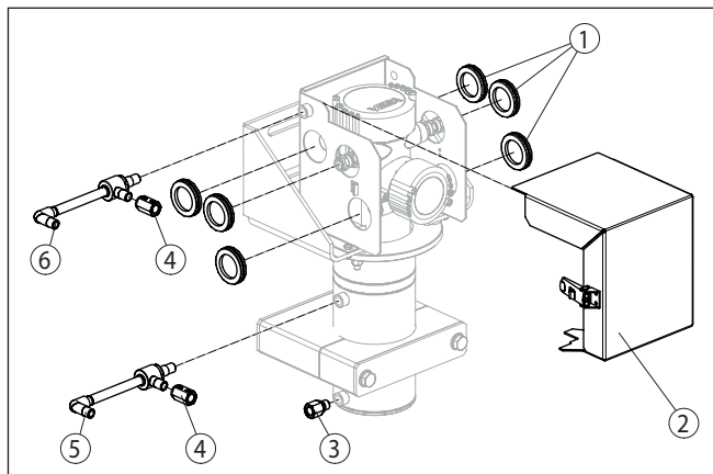
Fig. 16: Reservedelen - luchtkoeling SOLITRAC, POINTRAC
