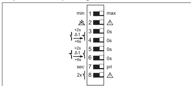
Fig. 3: DIL-schakelaar VEGATOR 131
