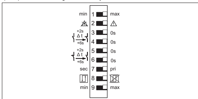
Fig. 4: Interruptor DIL VEGATOR 132
