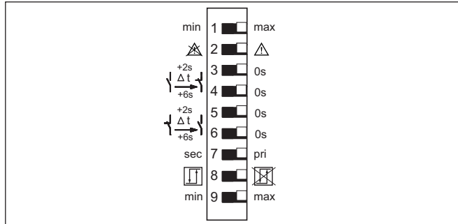
Fig. 4: Interruptor DIL VEGATOR 132
