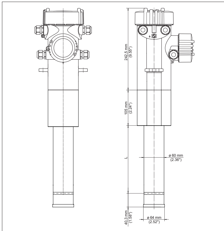
插图. 29: FIBERTRAC 32
