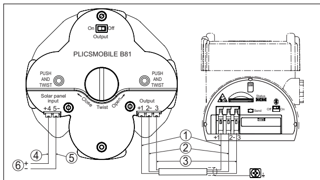
Fig. 12: Raccordement du PLICSMOBILE B81/S81
