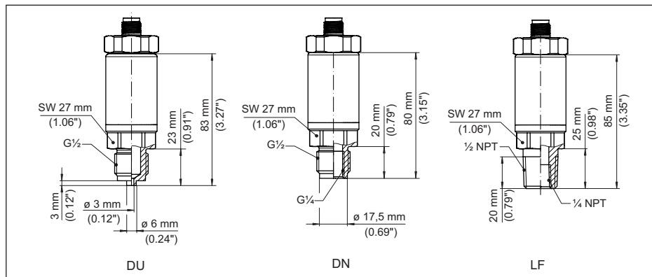
Fig. 18: VEGABAR 19, raccord fileté non arasant
