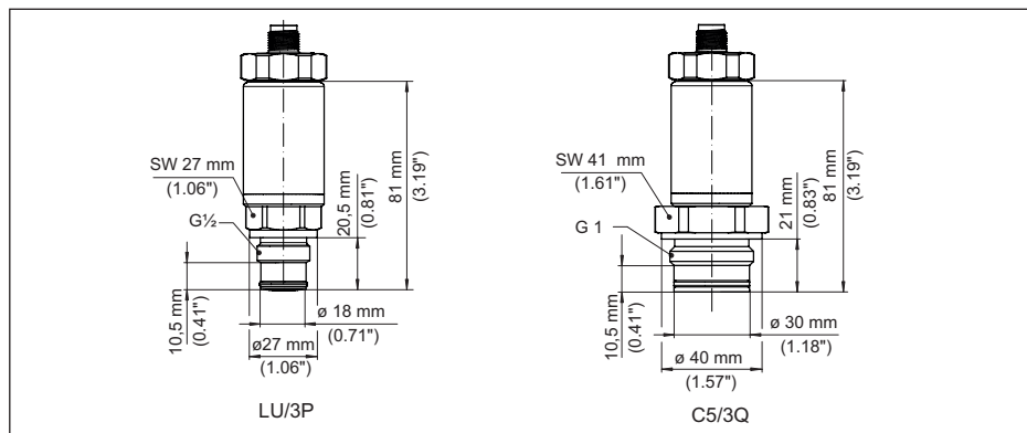
Fig. 19: VEGABAR 19, raccord fileté arasant
