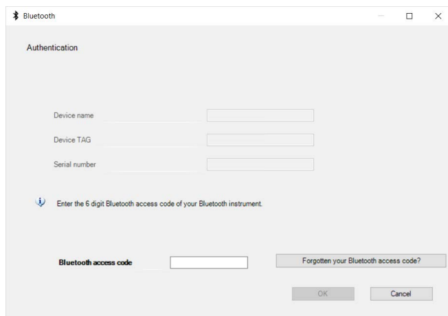
Fig. 22: Invoer Bluetooth-toegangscade
