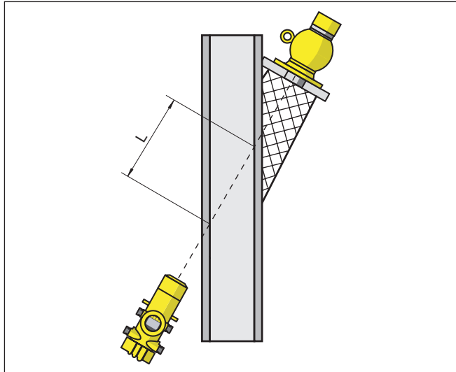
Fig. 19: With inclined mounting, the radiated length of the tube is applicable
