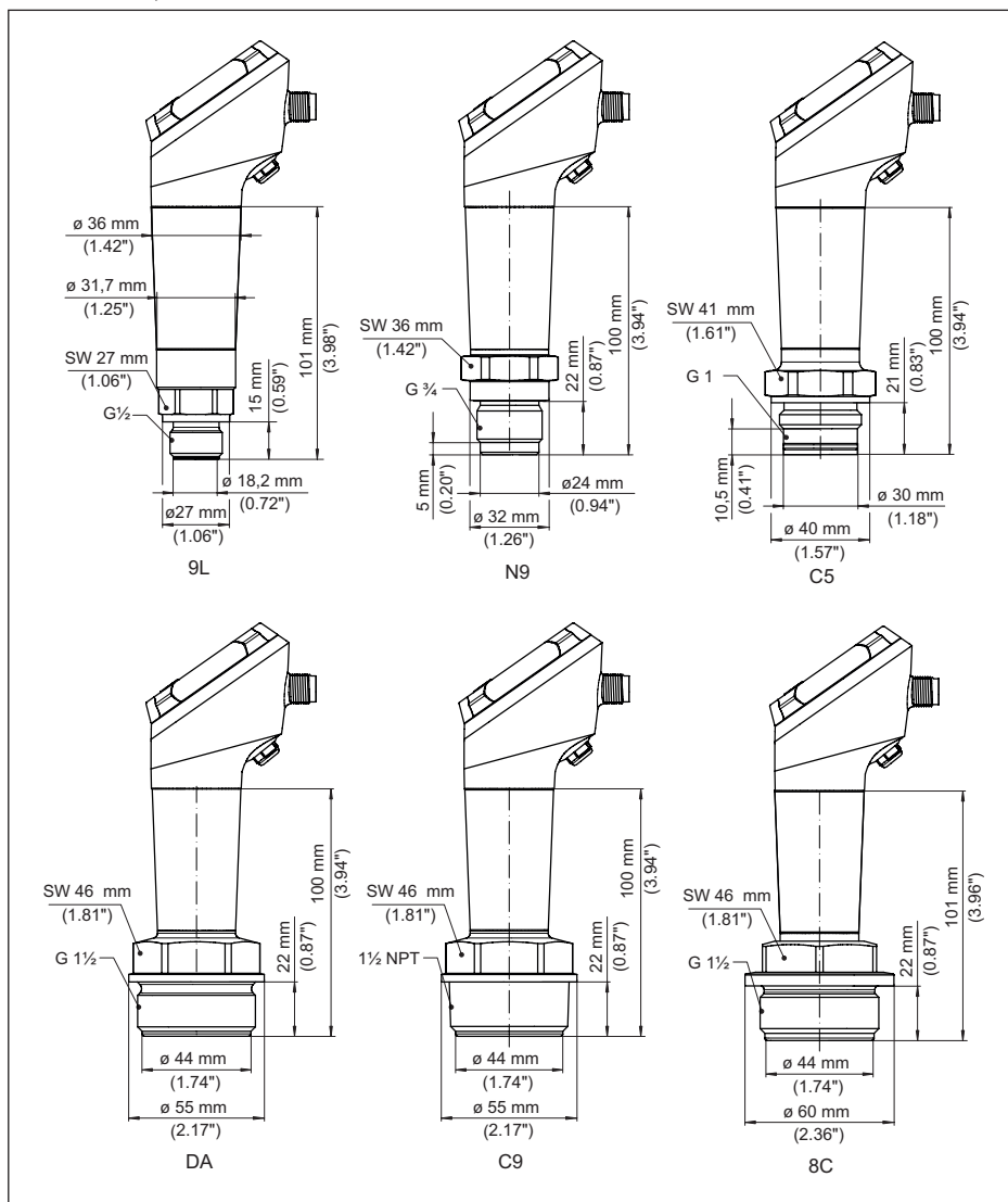
Fig. 35: VEGABAR 38, raccord fileté arasant
