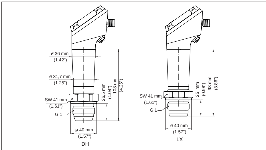
Fig. 36: VEGABAR 39, raccord cône/tube
