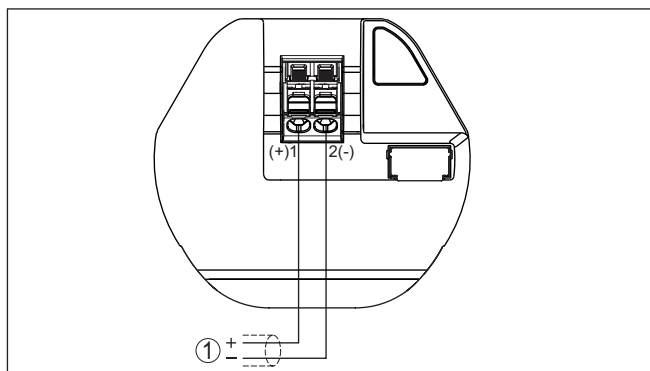
Fig. 20: Compartiment de raccordement VEGAPULS 21
