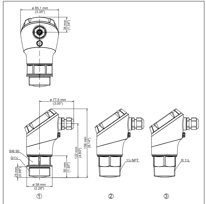
插图. 25: VEGAPULS 11, 21, 31 尺寸
