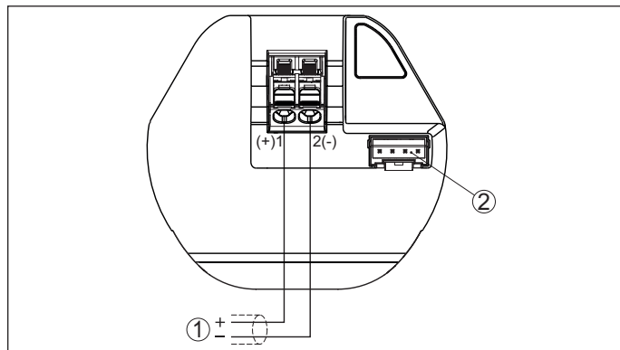
Fig. 15: Compartiment de raccordement VEGAPULS
