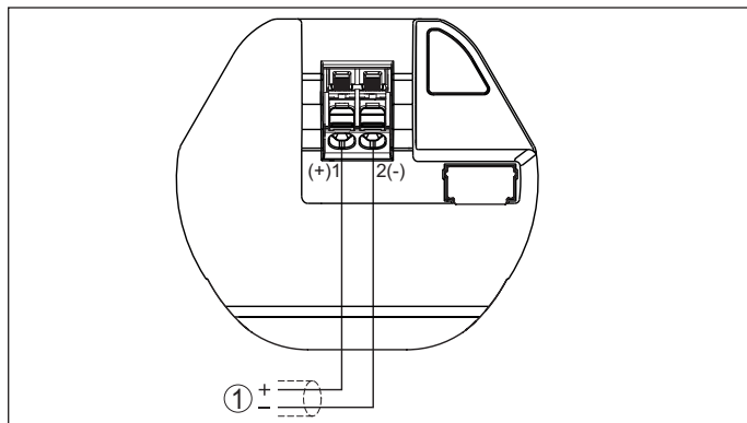
Fig. 13: Compartiment de raccordement VEGAPULS
