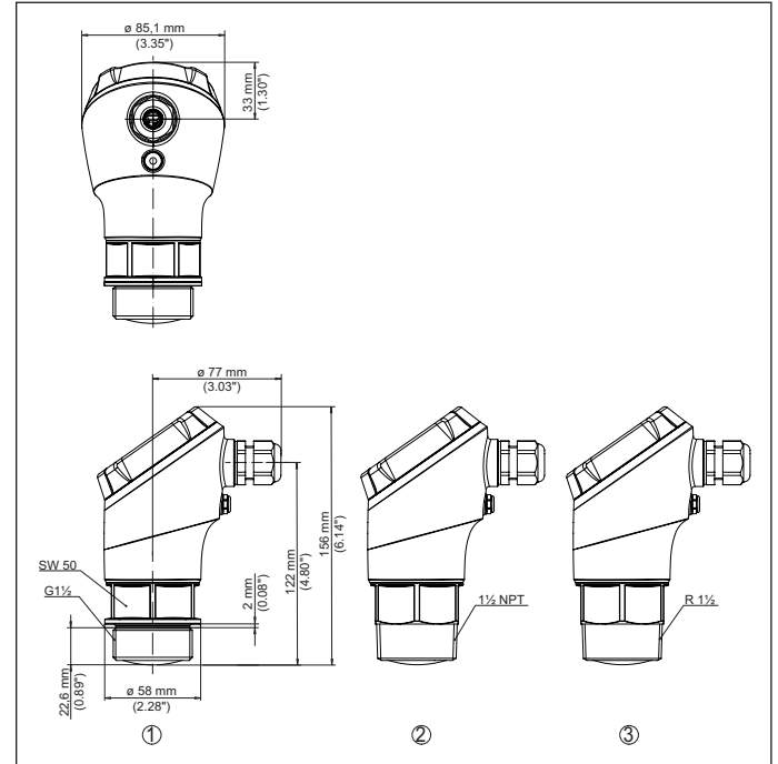
Fig. 25: Dimensions VEGAPULS 11, 21, 31
