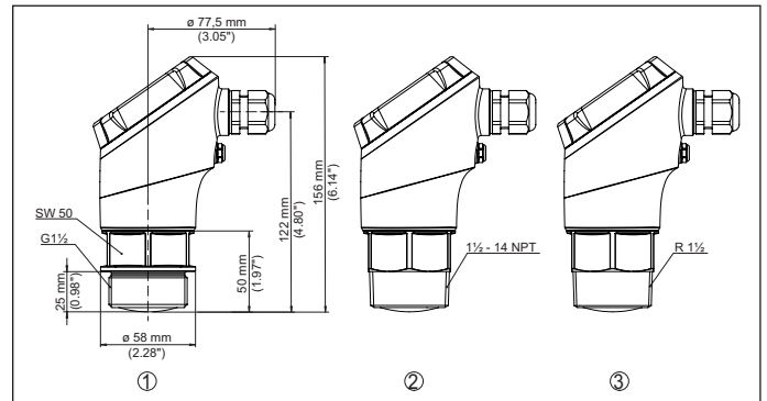
Figura 24: Dimensioni VEGAPULS 11, 21, 31
