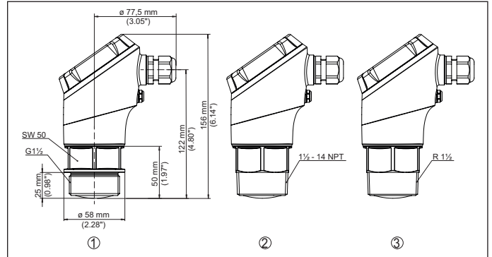
Fig. 24: Afmetingen VEGAPULS 11, 21, 31
