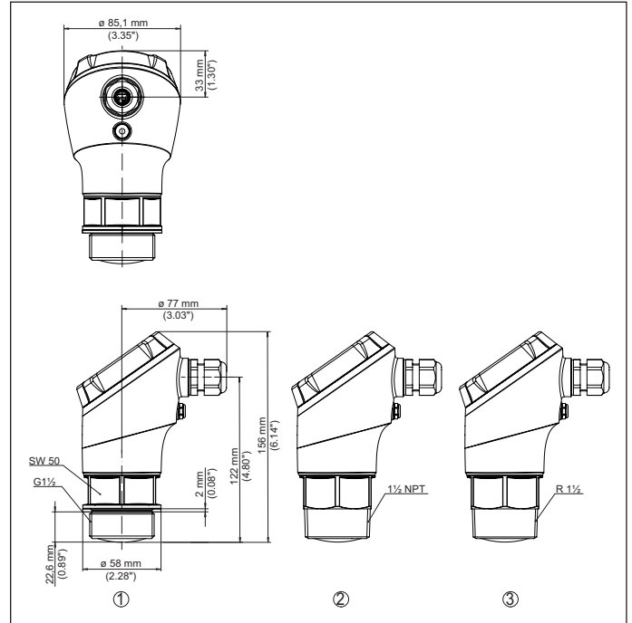
Fig. 25: Afmetingen VEGAPULS 11, 21, 31
