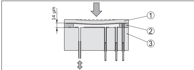
Fig. 1: Configuration of the Mini-CERTEC® measuring cell
