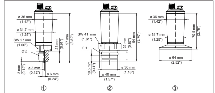
Fig. 25: Dimensions VEGABAR 29
