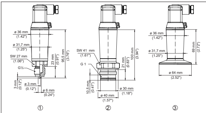
Fig. 24: Dimensions VEGABAR 28
