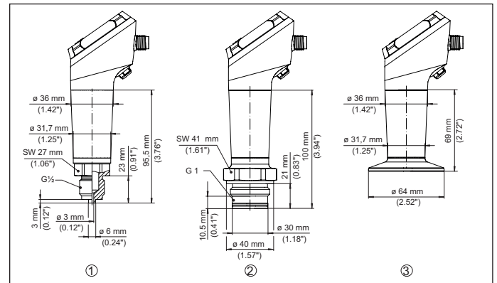
Fig. 26: Dimensions VEGABAR 38
