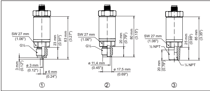
Fig. 22: Dimensions VEGABAR 18
