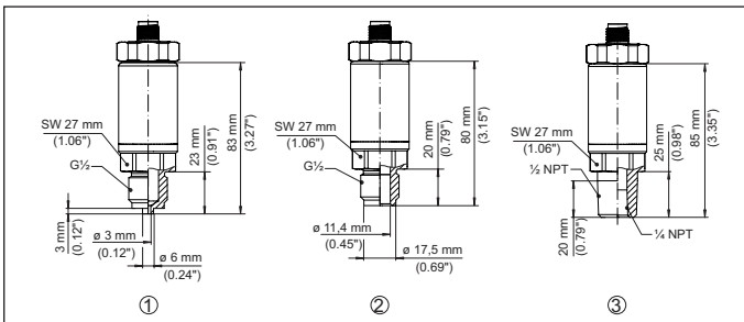
Fig. 23: Dimensions VEGABAR 19
