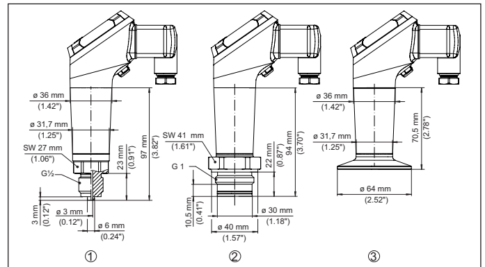
Fig. 27: Dimensions VEGABAR 39
