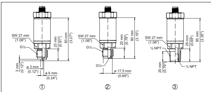
Fig. 23: Dimensions VEGABAR 19
