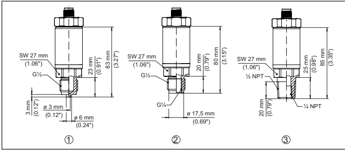
Fig. 22: Dimensions VEGABAR 18
