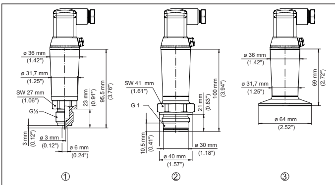
Fig. 24: Dimensions VEGABAR 28
