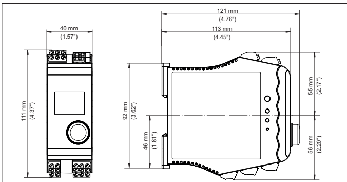
Fig. 17: Dimensions VEGAMET 142
