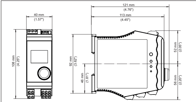
Fig. 16: Dimensions VEGAMET 141
