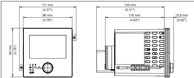
Fig. 18: Dimensions VEGAMET 341
