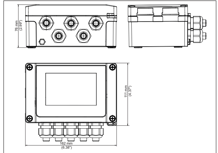
Fig. 20: Dimensions VEGAMET 841, 842
