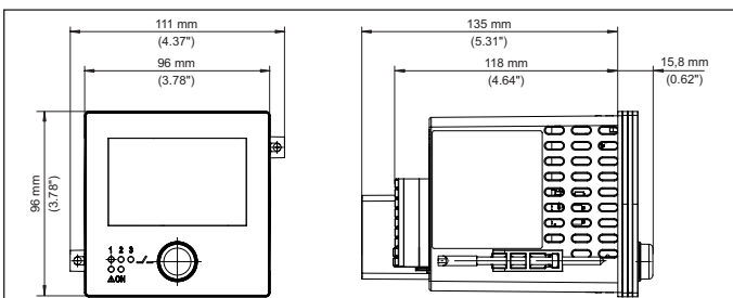
Fig. 19: Dimensions VEGAMET 342
