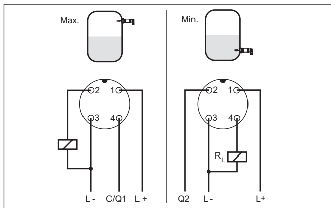
Fig. 8: Wiring plan (housing), terminal assignment IO-link output with M12 x 1 plug connection
