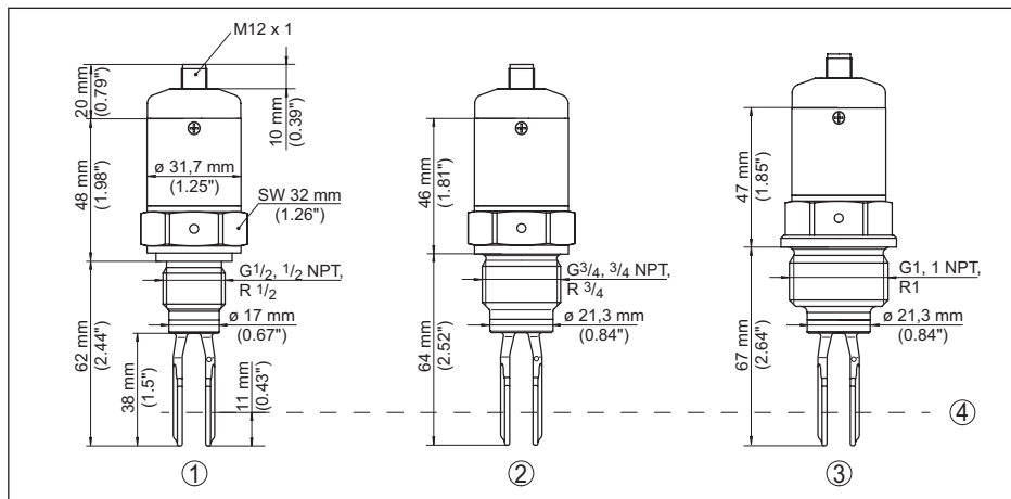
Fig. 12: VEGASWING 51, standard version - threaded fittings
