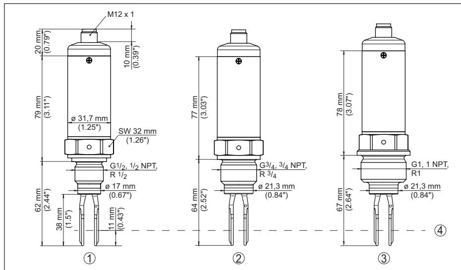
Fig. 13: VEGASWING 51, high temperature versions - threaded fittings
