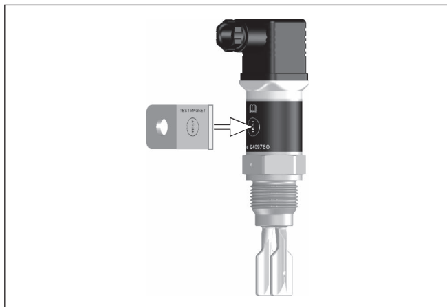
Fig. 15: Simulation of the output signal
