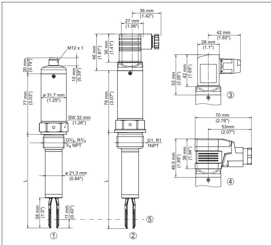
Fig. 19: VEGASWING 53, high temperature versions, threaded fittings
