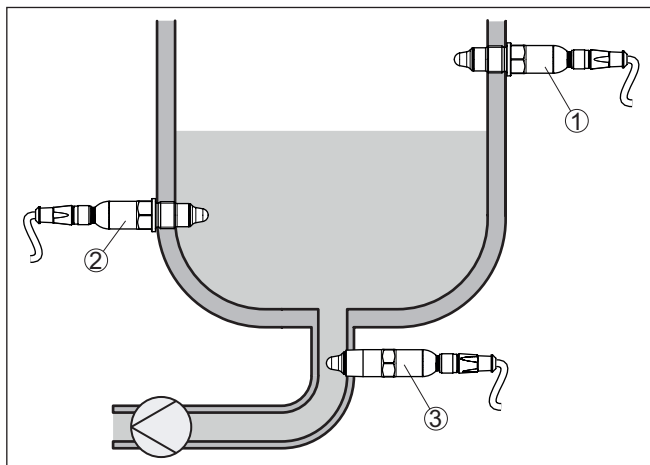
Fig. 3: Installation examples
