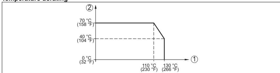
Abb. 2: Temperature derating VEGABAR 28, 29
