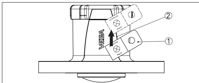
Fig. 14: Sensor activeren via magneet
