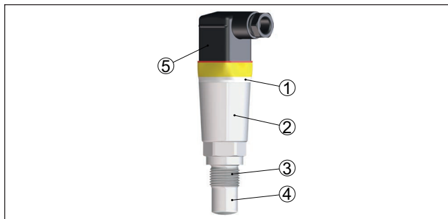
Fig. 1: VEGAPOINT 24
