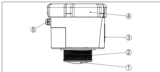
Fig. 6: Components of the radar sensor VEGAPULS Air 41 (example version with thread G1 1/2)
