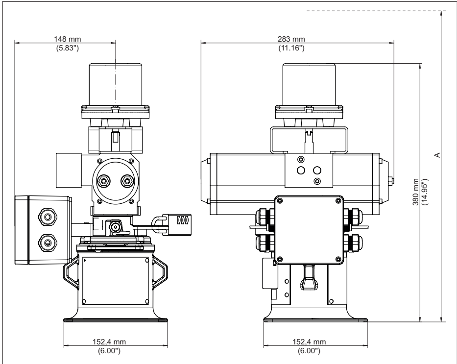
Fig. 43: Source holder VEGASOURCE 81, version B - Pneumatic ON/OFF switching with ON/OFF position switches
