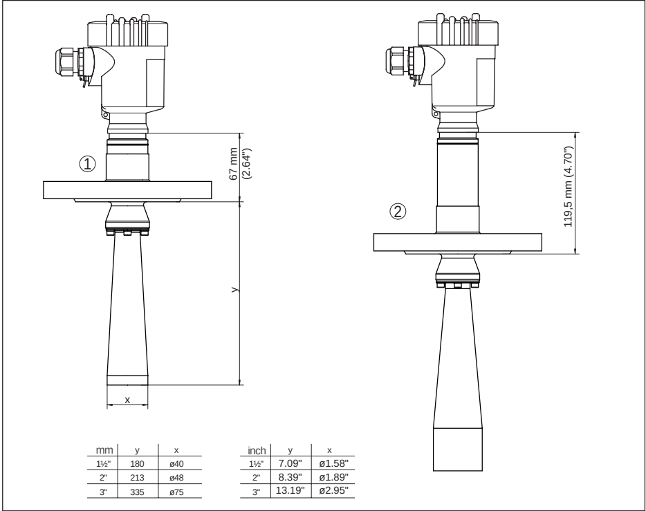
插图. 94: VEGAPULS 6X，带有号角天线的法兰，至 +150 °C (+302 °F)/+250 °C (+482 °F)
