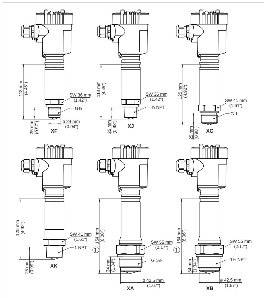
插图: 93: VEGAPULS 6X, 带有内置天线系统的螺纹至 +200 °C (+392 °F)/+250 °C (+482 °F)
