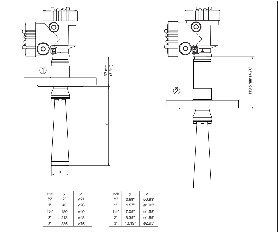
插图. 91: VEGAPULS 6X, 带有号角天线的法兰, 至 +150 °C (+302 °F)/+250 °C (+482 °F)
