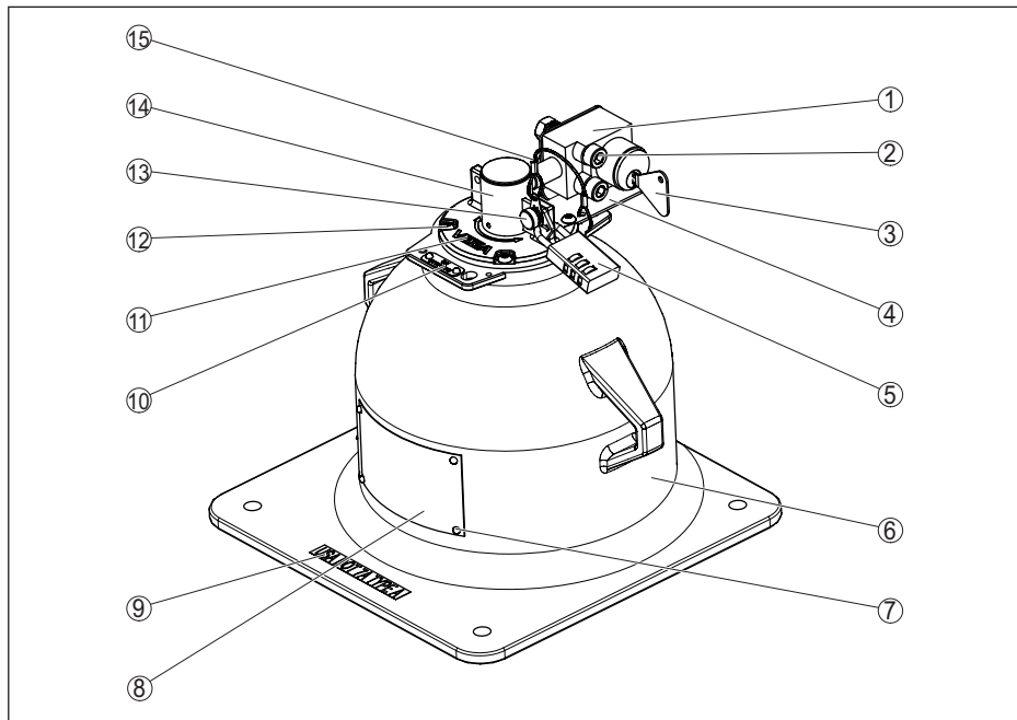
Fig. 35: Materials VEGASOURCE 83 - Version X, C - with Interlock switch
