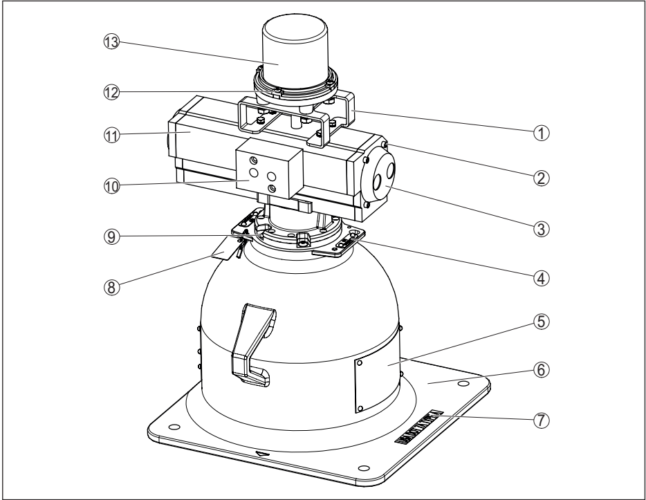
Fig. 36: Materials VEGASOURCE 83 - Version B
