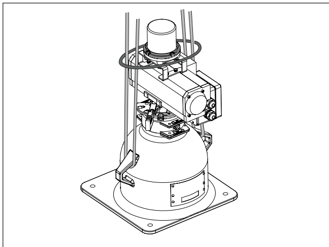
Fig. 8: Lifting of a source holder with pneumatic ON/OFF switching
