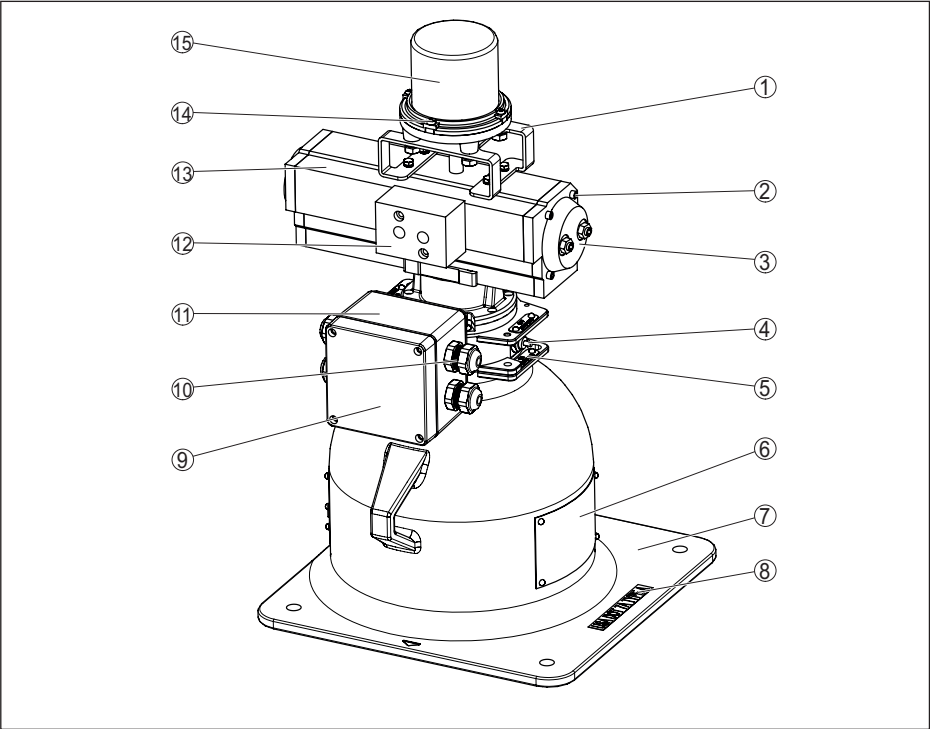
Fig. 37: Materials VEGASOURCE 83 - Version B - with ON/OFF position switches
