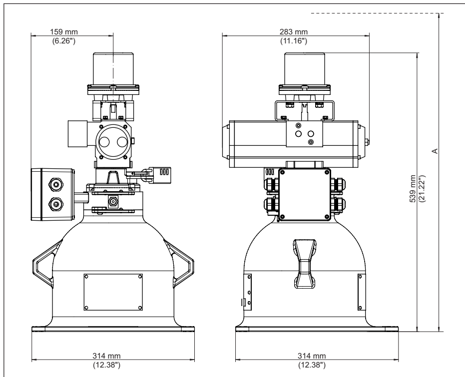
Fig. 42: Source holder VEGASOURCE 83, version B - Pneumatic ON/OFF switching with ON/OFF position switches
