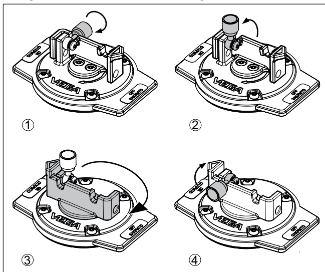
Fig. 26: Switching the radiation on - VEGASOURCE 83 version X, C
