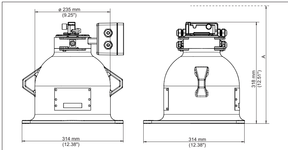
Fig. 39: Source holder VEGASOURCE 83, version X, C - Manual ON/OFF switching with ON/OFF position switches
