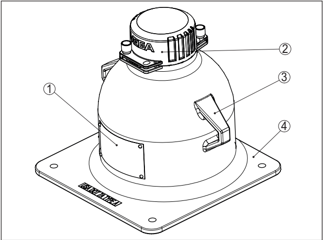
Fig. 6: Source holder VEGASOURCE 83
