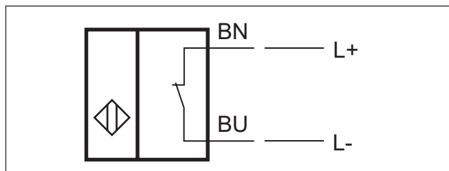
Fig. 25: Wiring plan - ON/OFF position switches - NAMUR
