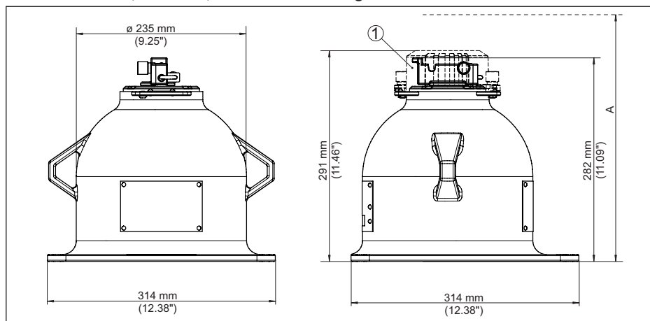
Fig. 38: Source holder VEGASOURCE 83, version X, C - Manual switching ON/OFF
