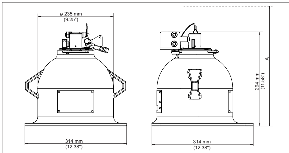
Fig. 40: Source holder VEGASOURCE 83, version X, C - Manual ON/OFF switching with Interlock switch
