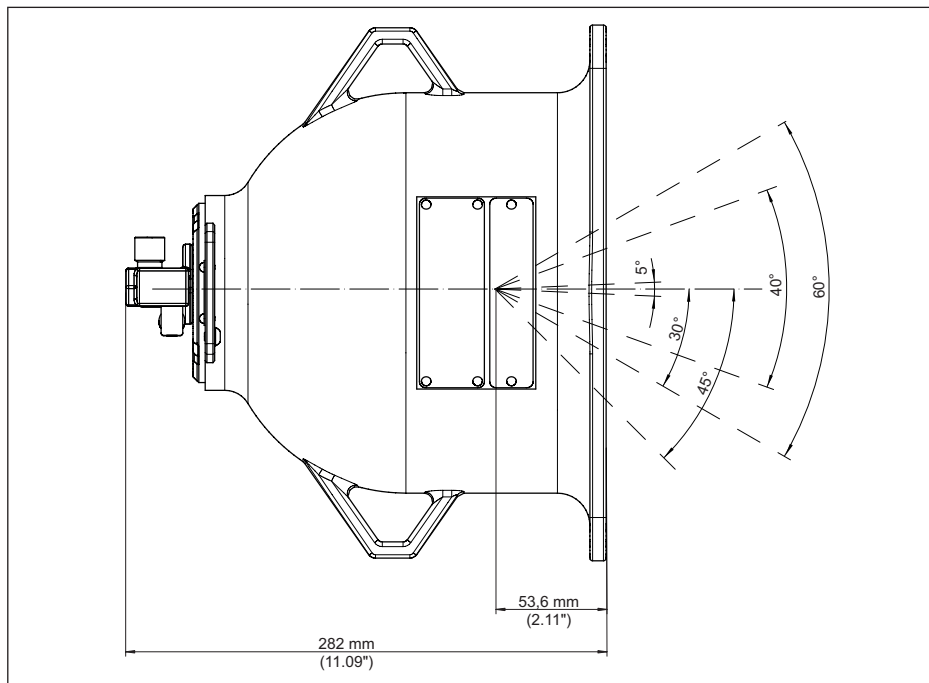
Fig. 43: Beam exit channel (e.g. version X, C)
