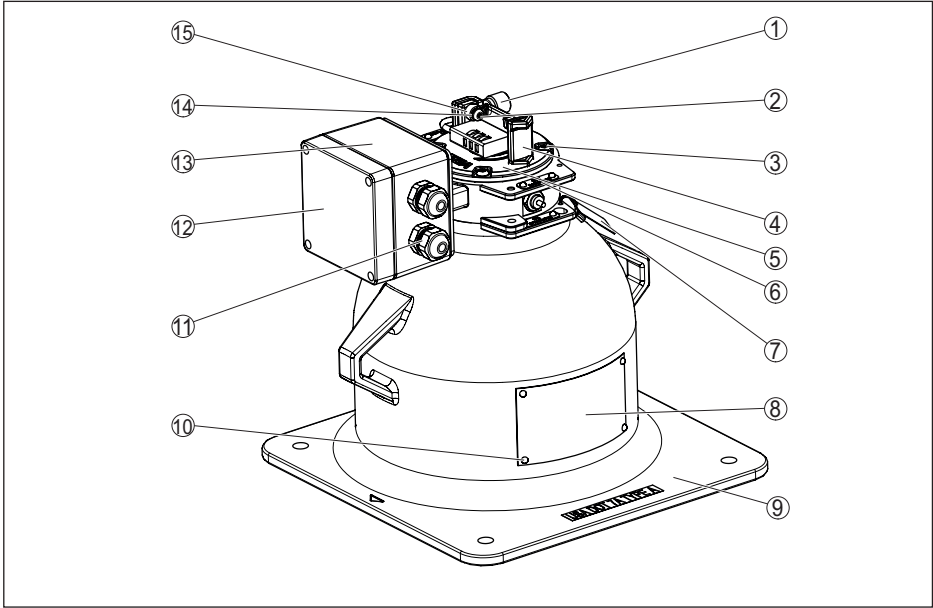
Fig. 34: Materials VEGASOURCE 83 - Version X, C - with ON/OFF position switches
