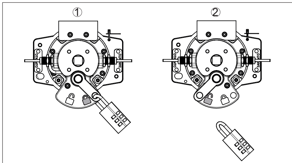
Fig. 30: Indication of the switching status with VEGASOURCE 83 - Version B - Pneumatic switching ON/OFF
