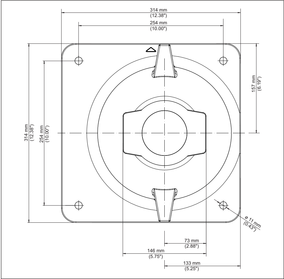
Fig. 44: Base plate with holes (e.g. version X, C)
