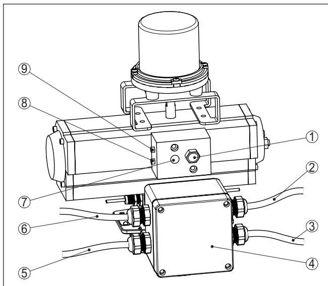
Fig. 23: Connection of the pneumatic lines on VEGASOURCE 83 - version B
