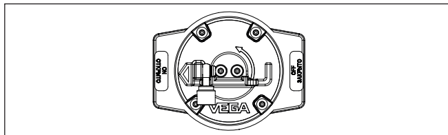
Fig. 27: Radiation "ON" - VEGASOURCE 83 Version X, C
