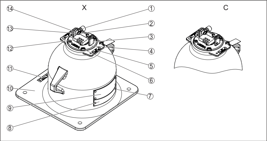
Fig. 33: Materials VEGASOURCE 83 - Version X, C
