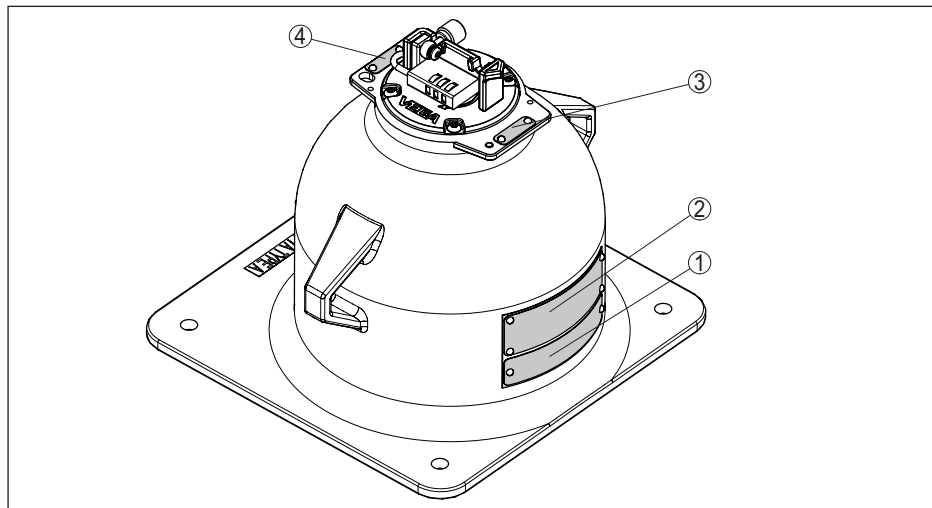
Fig. 3: Position of the type labels, e.g. version X, C - Manual switching ON/OFF
