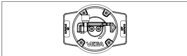
Fig. 28: Rayonnement "OFF" - VEGASOURCE 83 Version X, C
