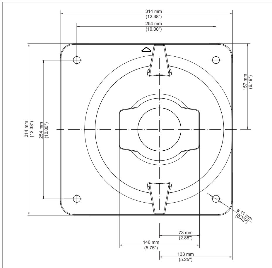
Fig. 44: Plaque de base perçages (par ex. version X, C)
