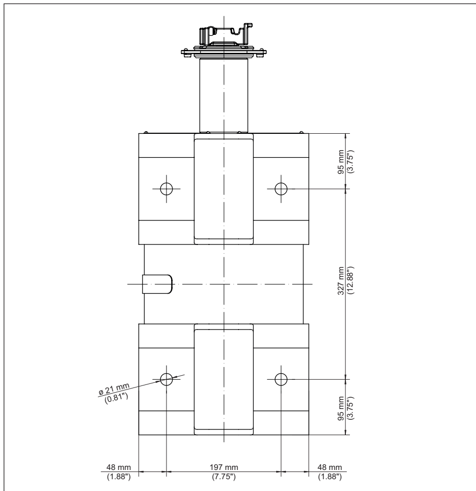
Fig. 26: Plaque de base perçages (par ex. version X, C)
