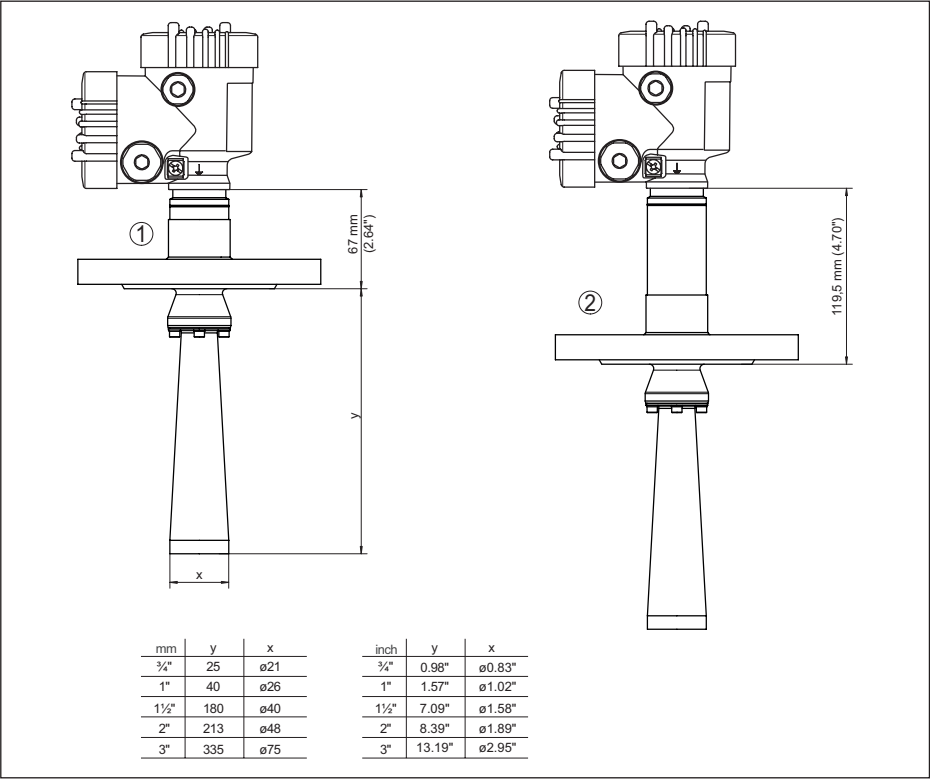
插图. 89: VEGAPULS 6X, 带有号角天线的法兰, 至 +150 °C (+302 °F)/+250 °C (+482 °F)
