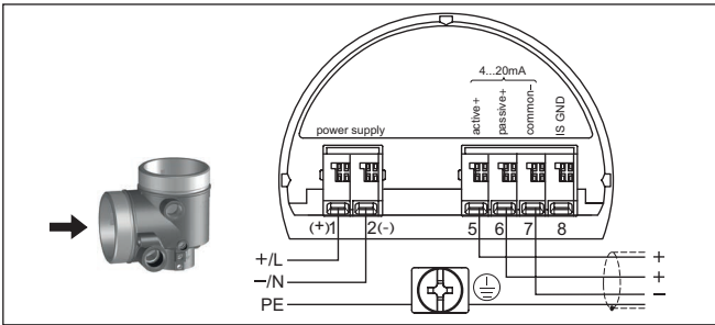
插图. 8: 电网供电时双腔式外壳的接线腔
