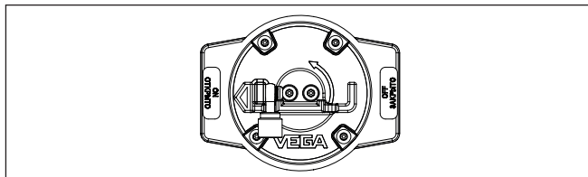
Fig. 17: Radiation "ON" - VEGASOURCE 86 Version X, C
