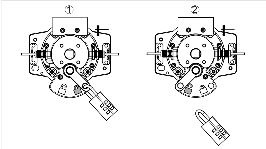
Fig. 20: Indication of the switching status with VEGASOURCE 86 - Version B - Pneumatic switching ON/OFF
