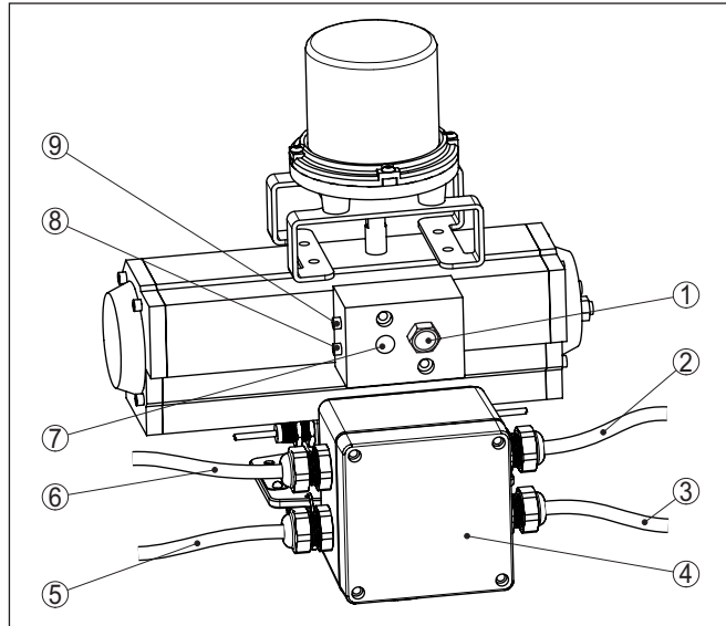
Fig. 13: Connection of the pneumatic lines on VEGASOURCE 86 - version B
