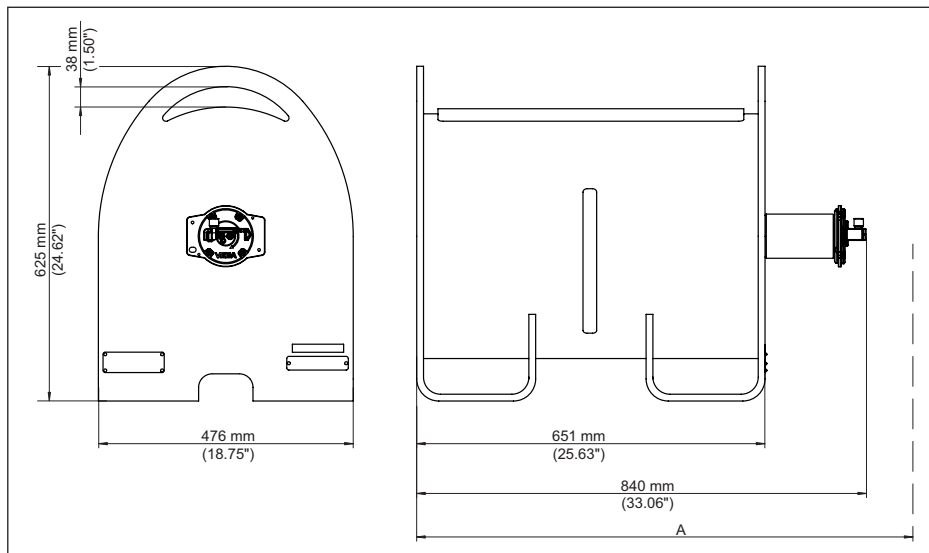
Fig. 24: Source holder VEGASOURCE 86, version X, C - Manual switching ON/OFF
