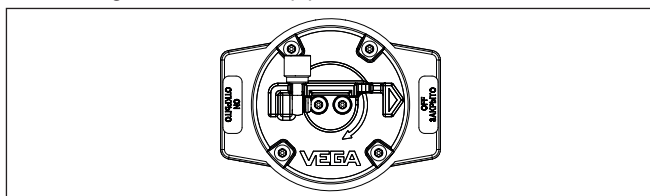
Fig. 18: Radiation "OFF" - VEGASOURCE 86 Version X, C
