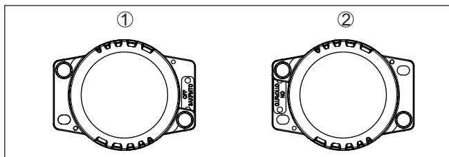
Fig. 19: Position indication with protective cap - VEGASOURCE 86 Version X, C
