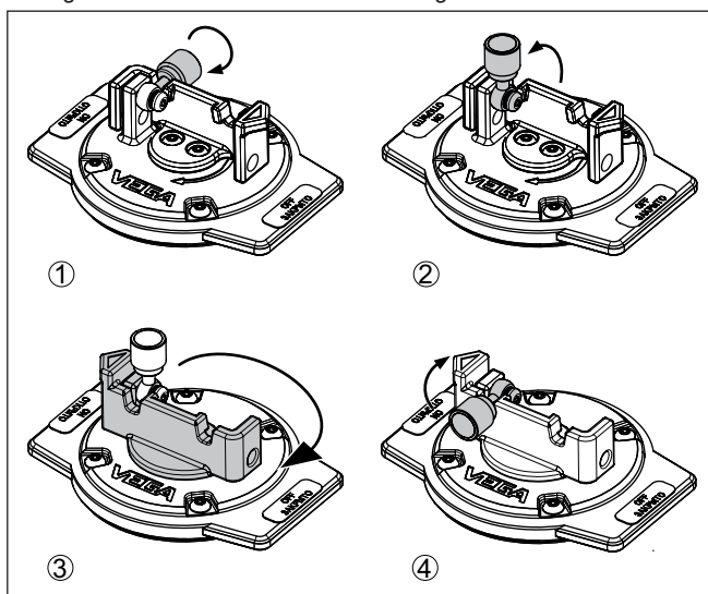
Fig. 16: Switching the radiation on - VEGASOURCE 86 version X, C
