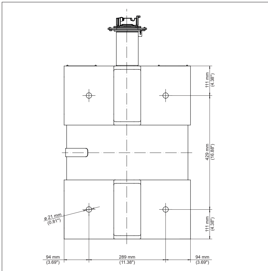
Fig. 24: Plaque de base perçages (par ex. version X, C)
