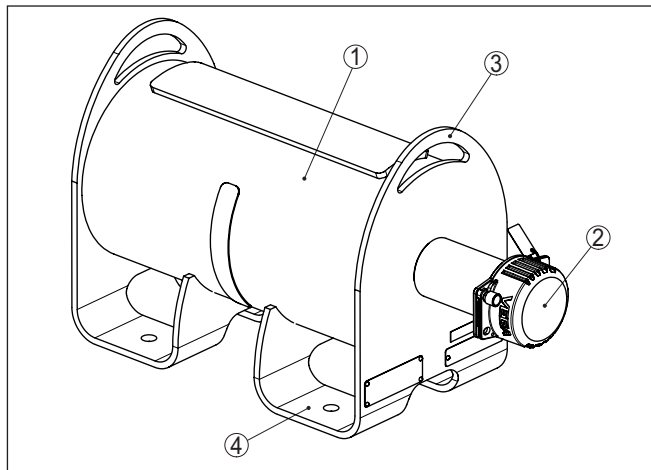
Fig. 4: Conteneur blindé VEGASOURCE 86
