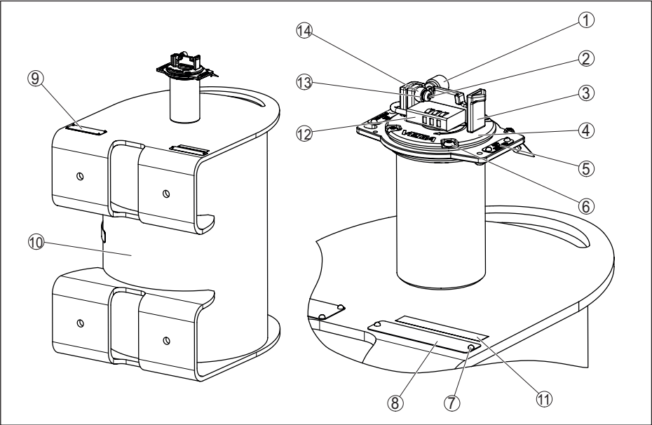
Fig. 23: Matériaux VEGASOURCE 86 - version X, C
