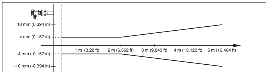
Fig. 36: Meetafwijking VEGASON 61
