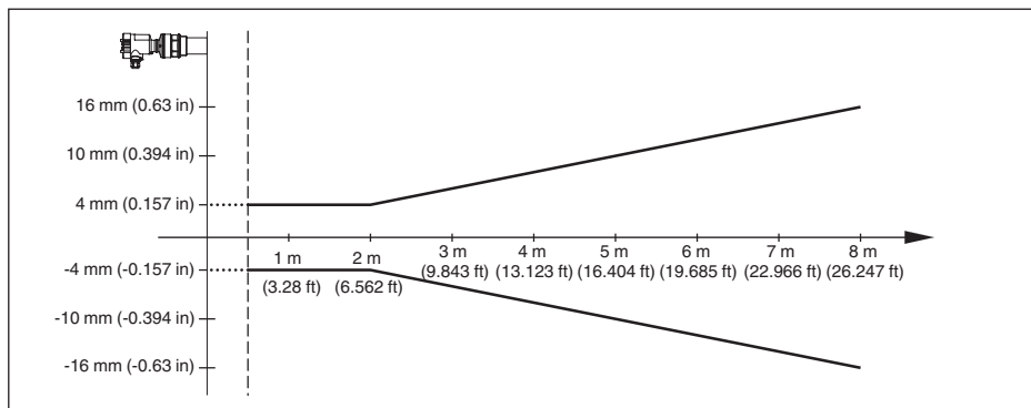
Fig. 34: Meetafwijking VEGASON 62
