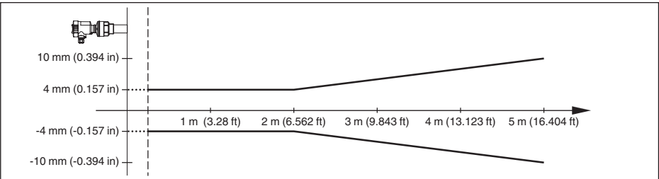
Fig. 31: Meetafwijking VEGASON 61
