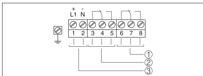
Fig. 9: Wiring plan, single chamber housing
