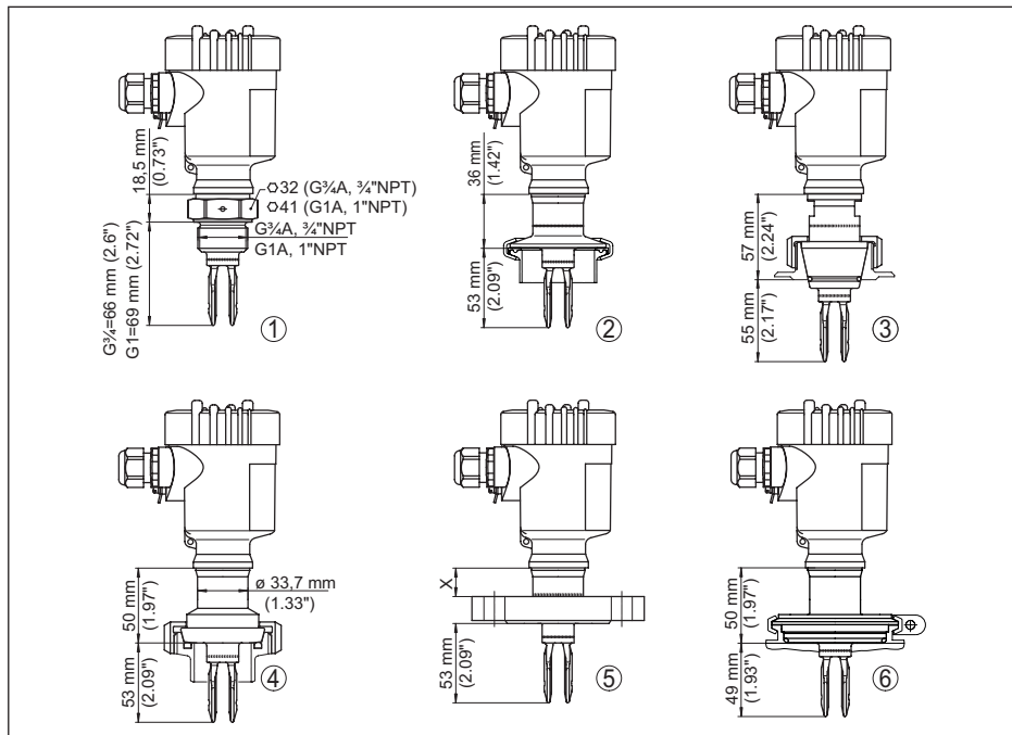
Rys. 18: VEGASWING 61
