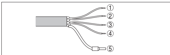
Fig. 11: Wire assignment connection cable. The numbers of the wires correspond to the terminals of the instrument.
